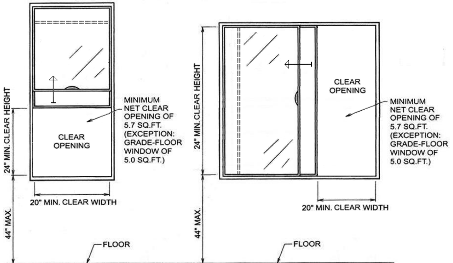
EMERGENCY ESCAPE WINDOW
