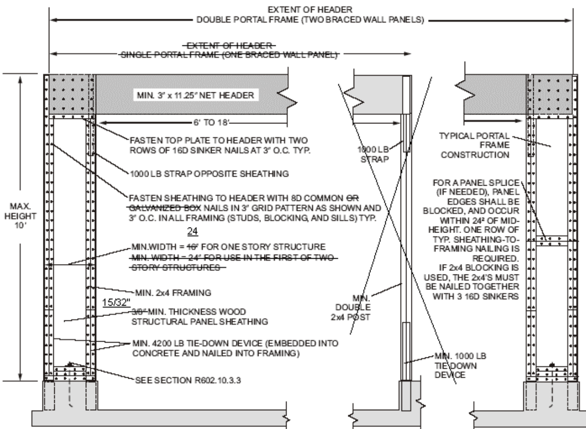
FIGURE R602.10.3.3
