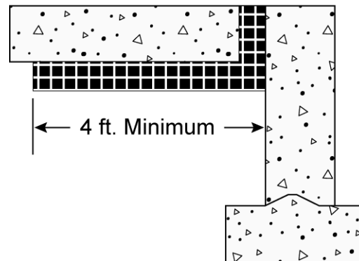
Beneath Slab Insulation
