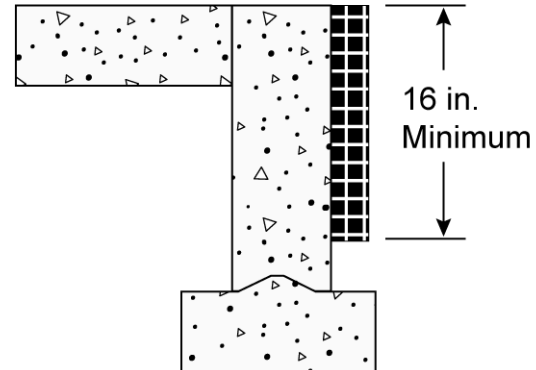
Outside Insulation
