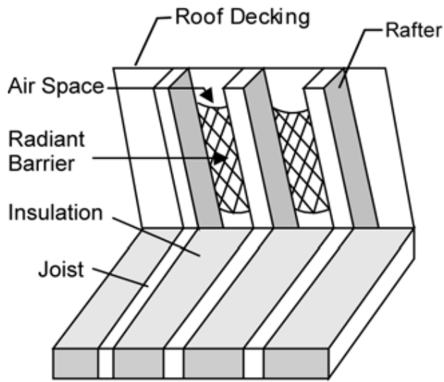
Method 1: Radiant Barrier Draped Over Top of Truss/Rafter
