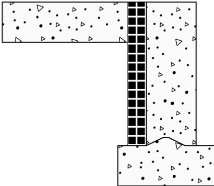
Inside Insulation
