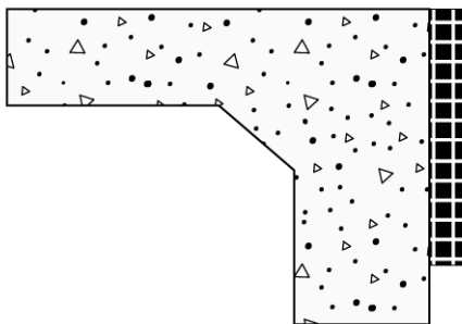
Monolithic Slab Insulation
