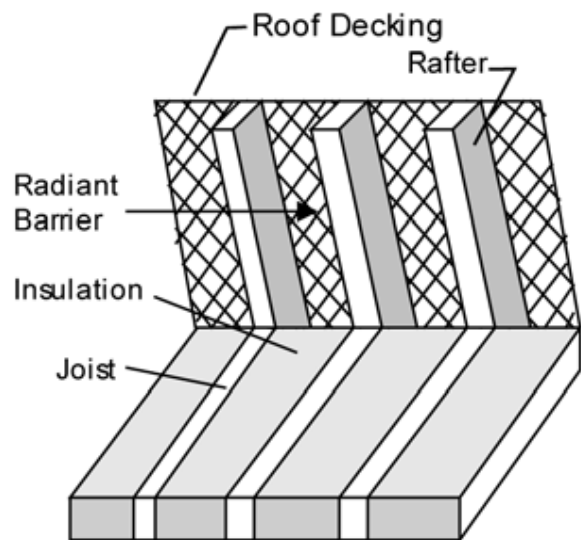
Method 4: Radiant Barrier Attached to Underside of Roof Deck
