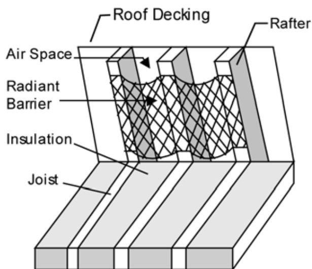
Method 3: Radiant Barrier Attached to Bottom of Truss/Rafter
