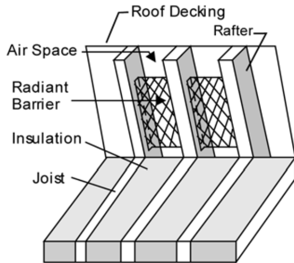
Method 2: Radiant Barrier Attached Between Truss/Rafters
